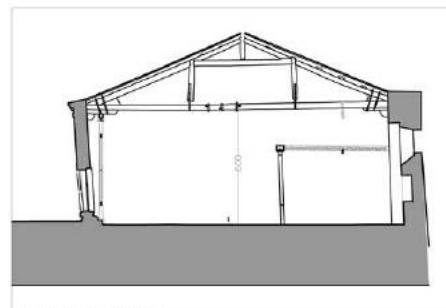
CROSS SECTION C-C'
